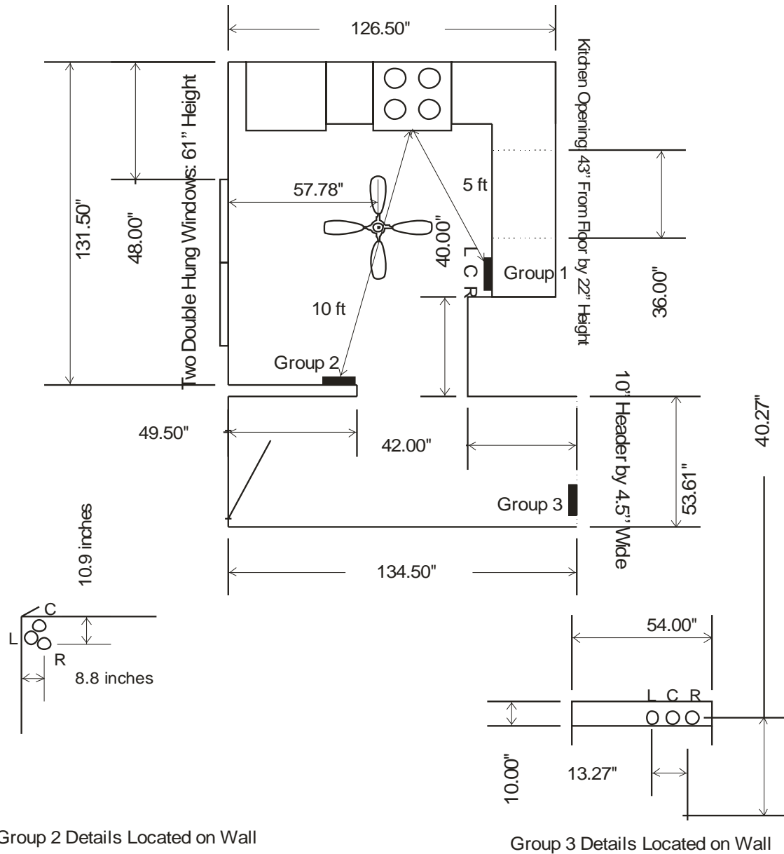
Figure A.8-2 Floor Layout for Test Home 8
