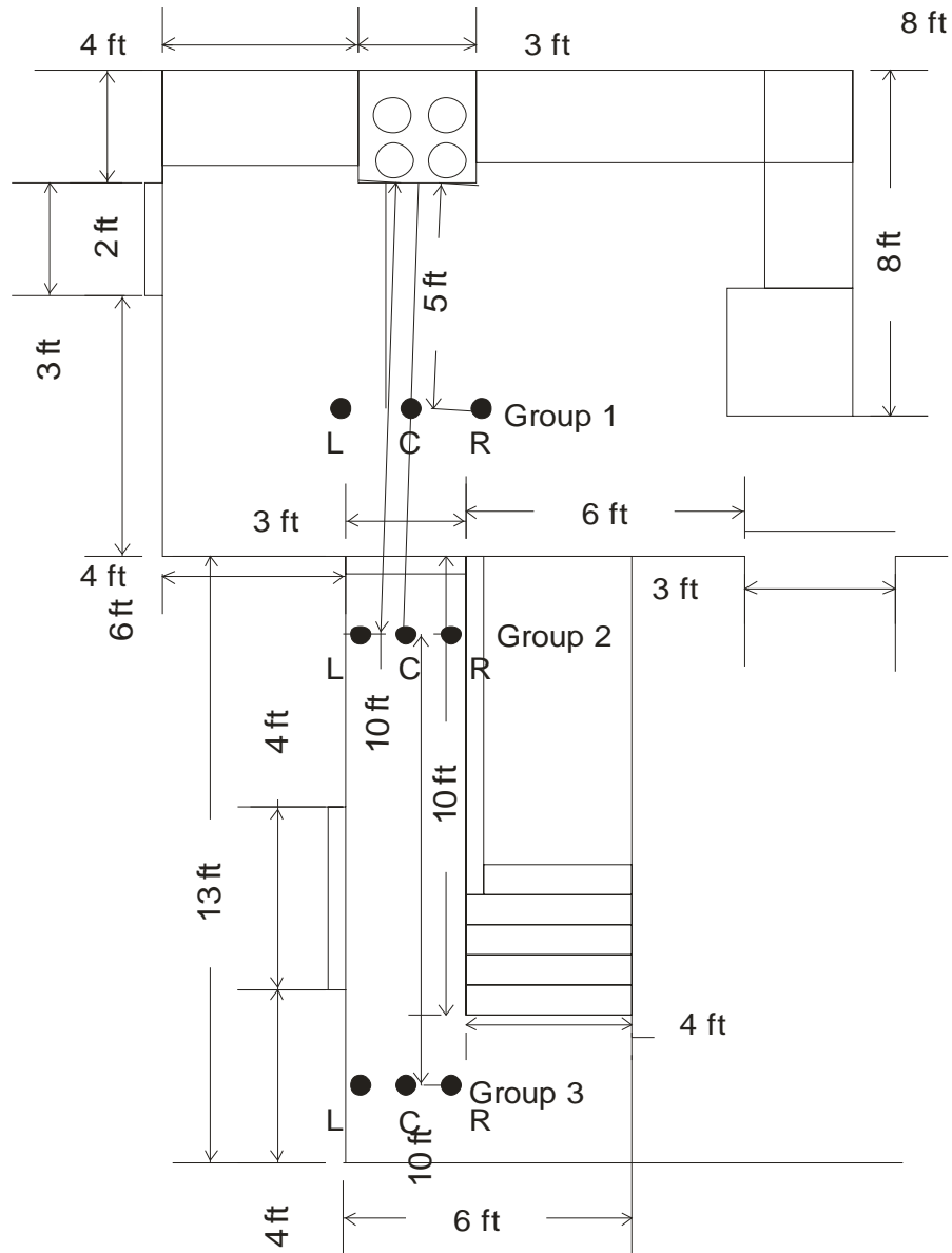
Figure A.3-2 Floor Layout for Test Home 3
