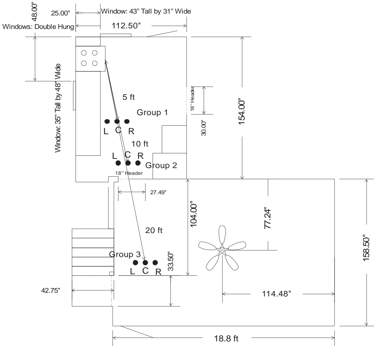
Figure A.7-2 Floor Layout for Test Home 7
