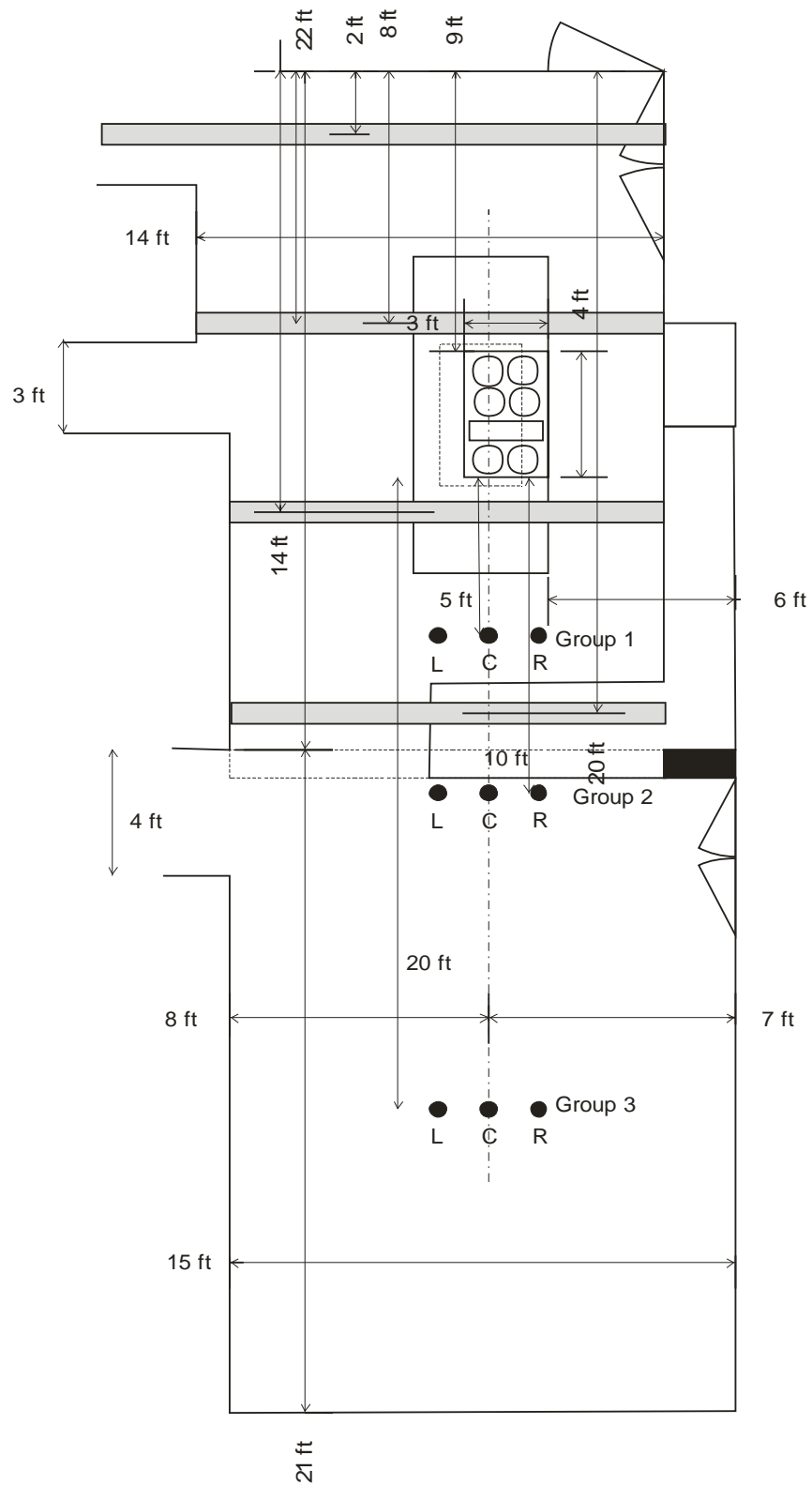
Figure A.2-2 Floor Layout for Test Home 2
