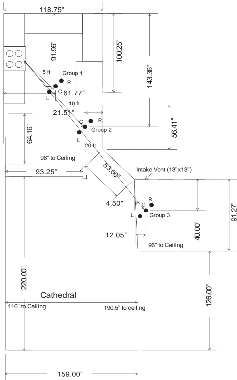
Figure A.6-2 Floor Layout for Test Home 6
