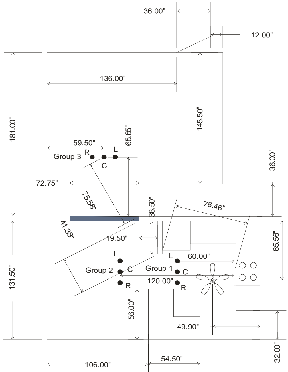
Figure A.5-2 Floor Layout for Test Home 5
