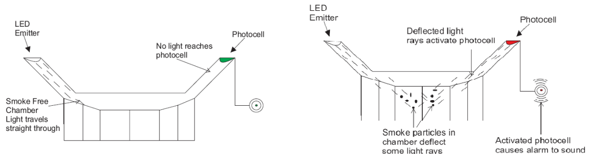
Figure 2. Photoelectric Chamber
