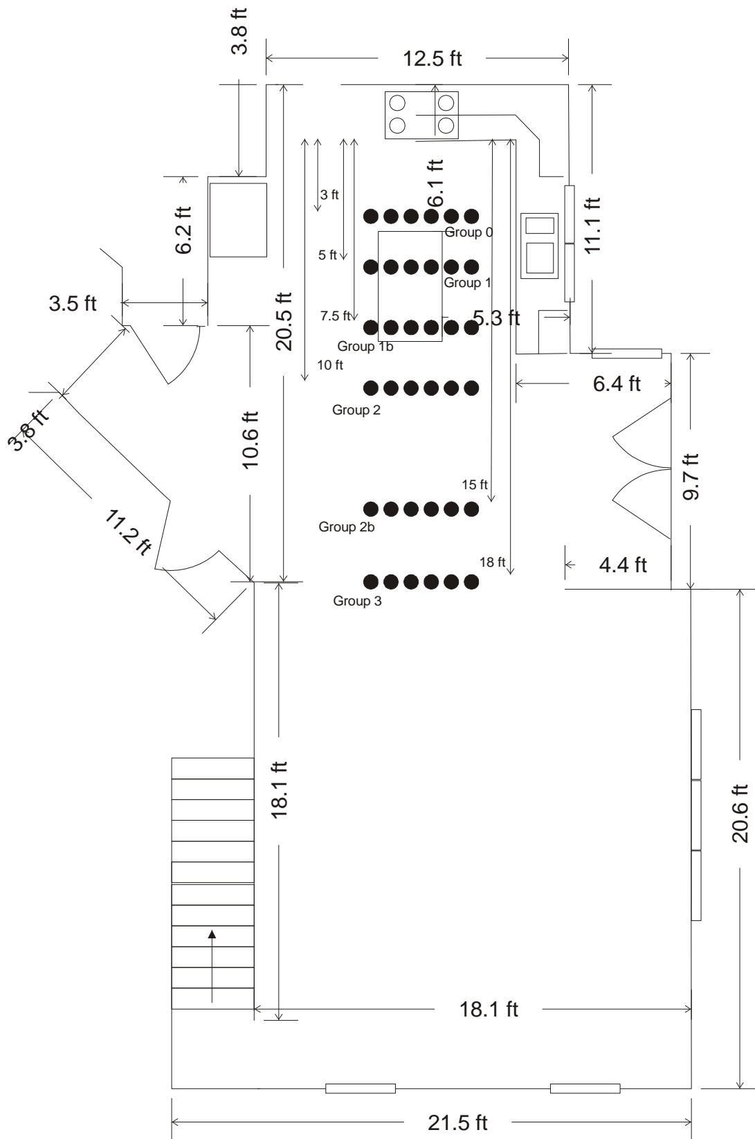
Figure A.9-2 Floor Layout for Test Home 9
