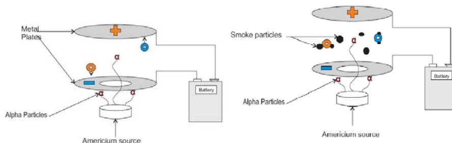
Figure 1. Ionization Chamber
