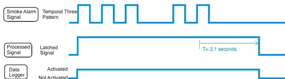
Figure 5. Conditioned Signal from the Smoke Alarm
