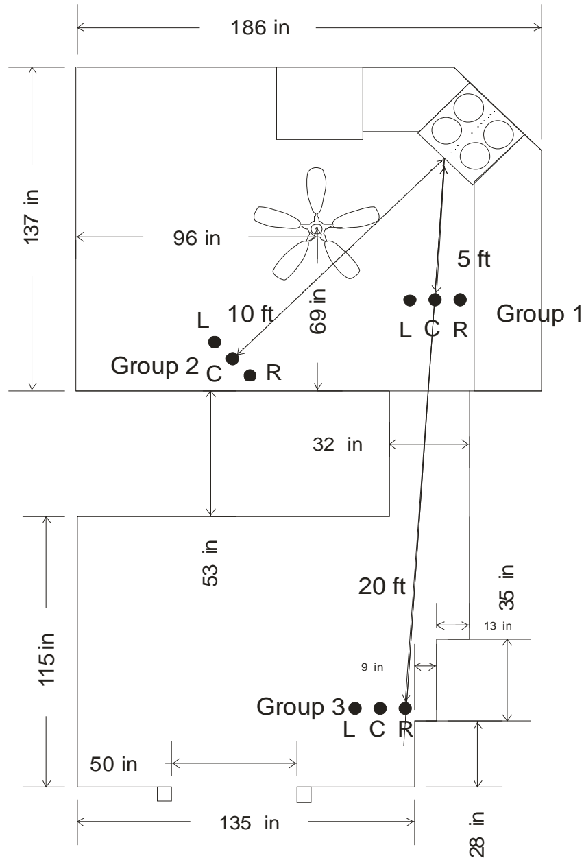
Figure A.4-2 Floor Layout for Test Home 4
