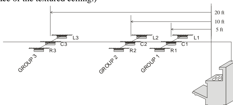
Figure 6. Test Setup for Homes 1-8
